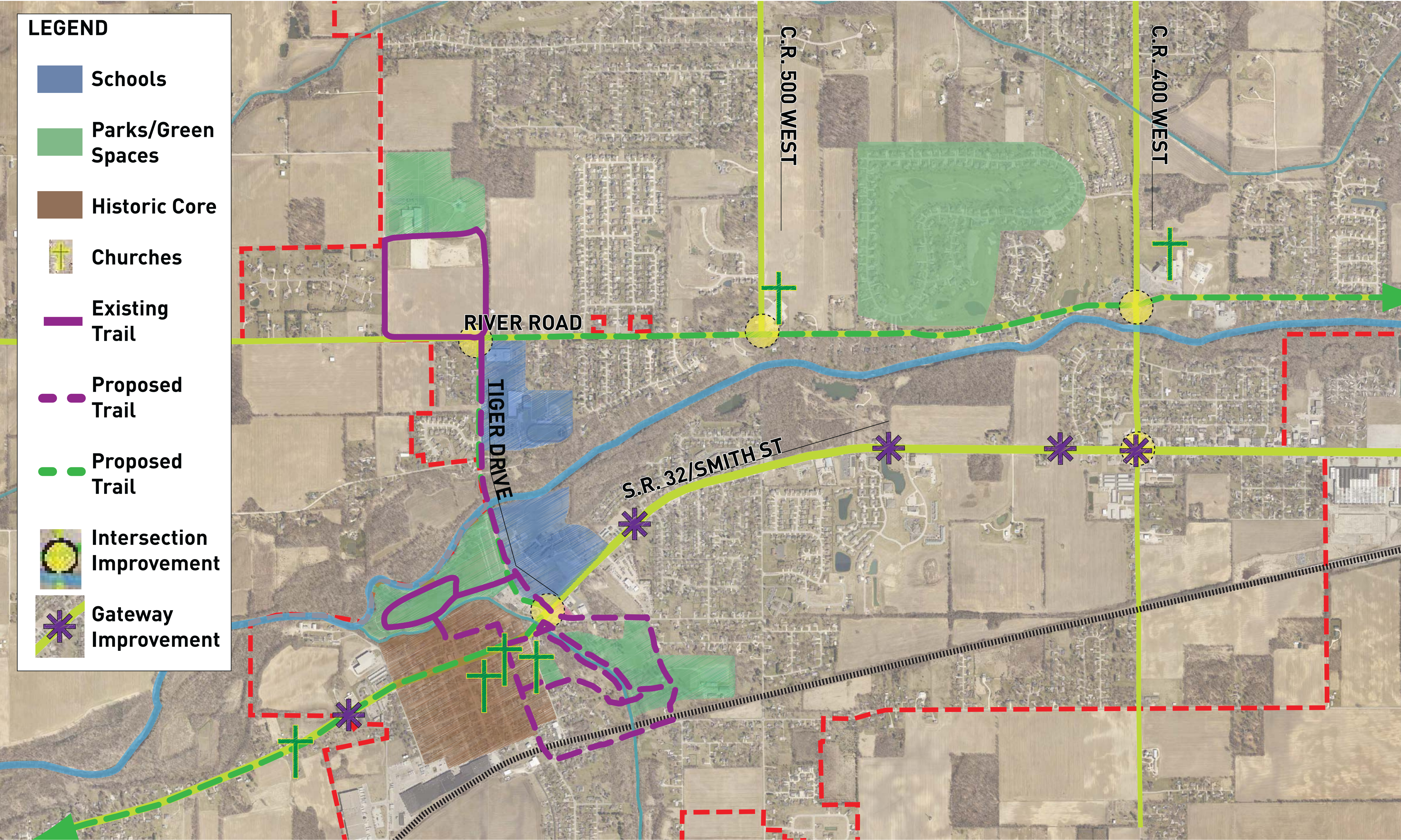
Yorktown Downtown Improvements-Cultural Amenities and Proposed Improvements
